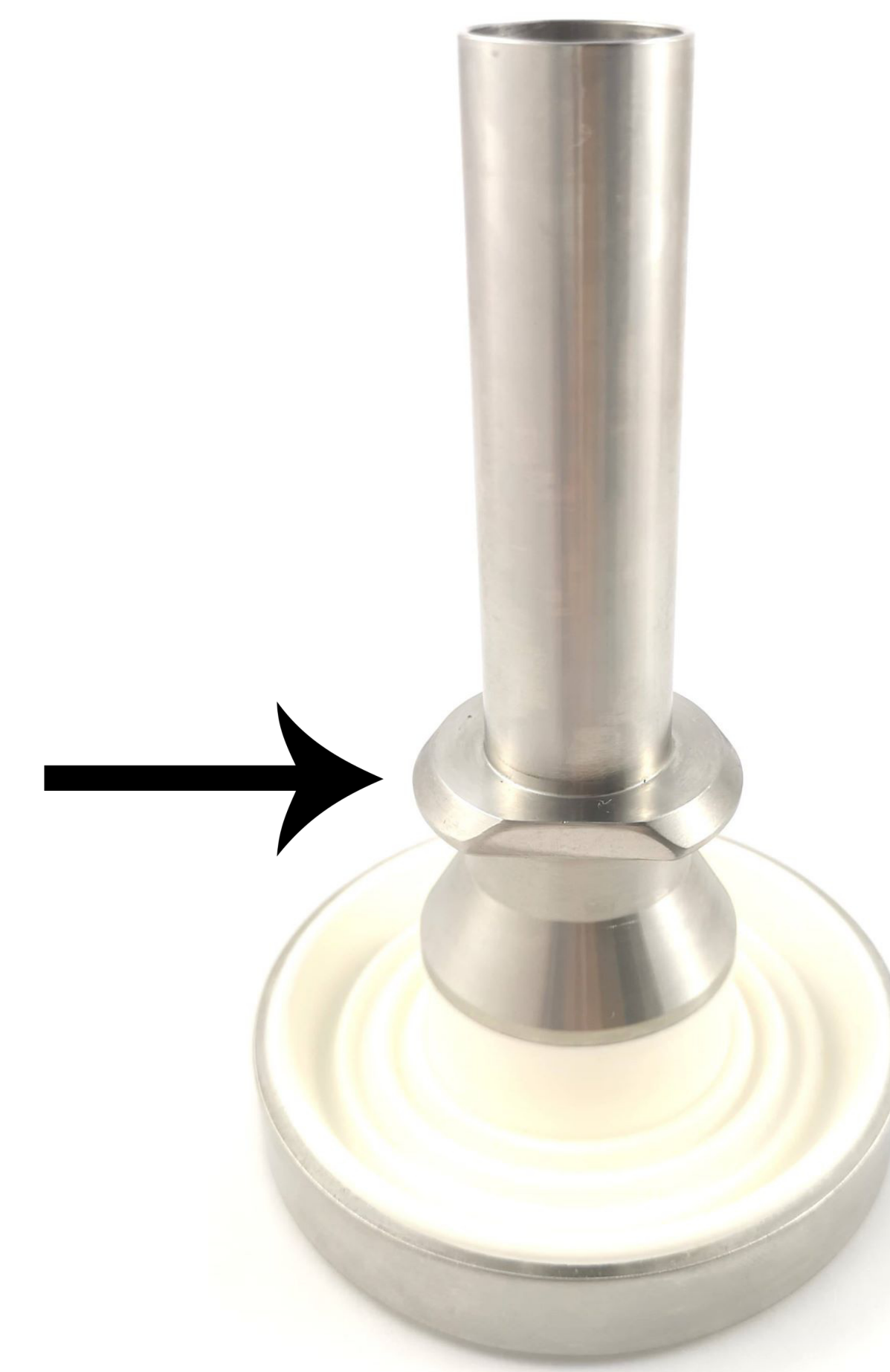
2. Filler membrane (18 mm) Flange height = 0.177 inch UMS-04253247102
