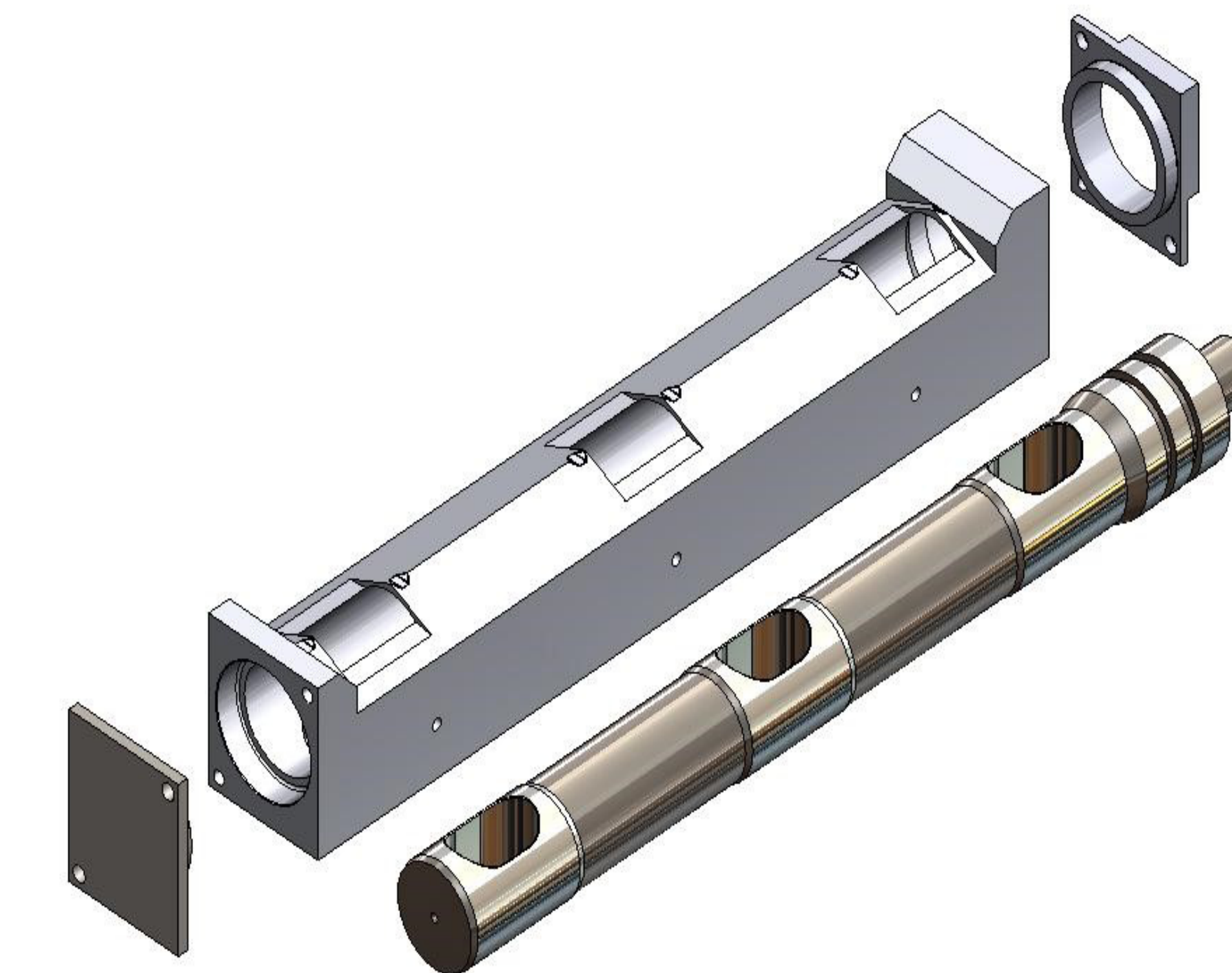
Refurbished dosing block (small)
