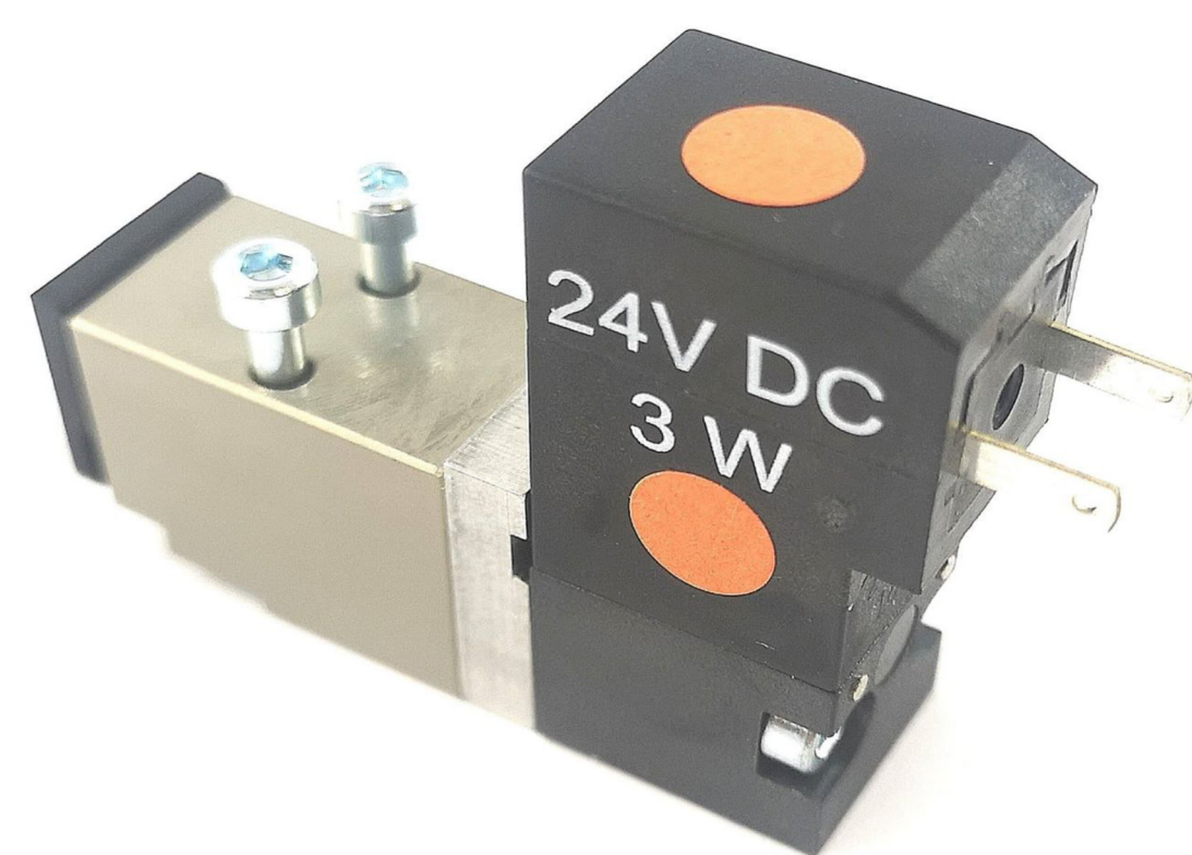
Pilot valve P1 & P2 (red dot) UMK-50363507
