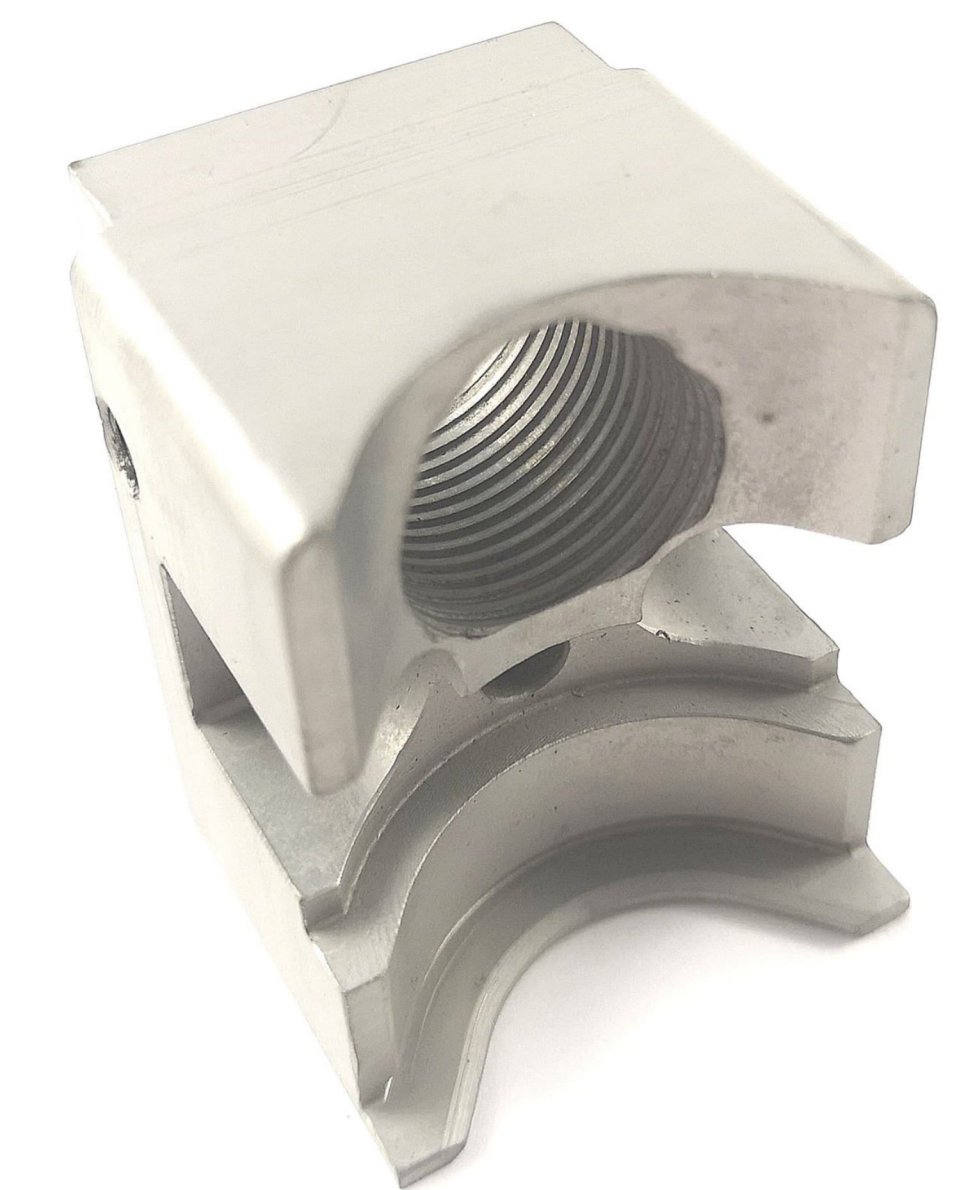
Mandrel support blow station UMK-94137018
