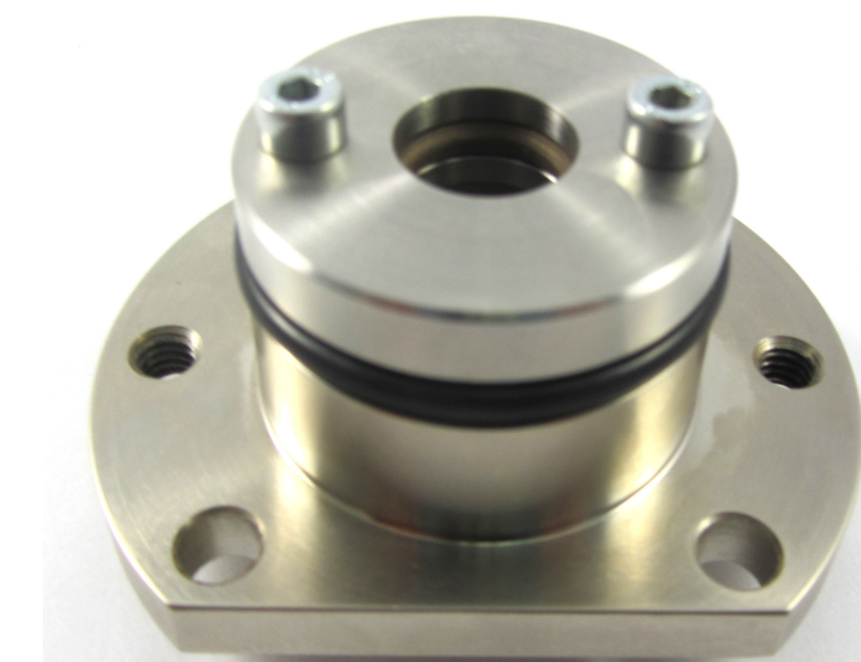
Sealing cartridge Assy (14 mm) UMK-95140265
