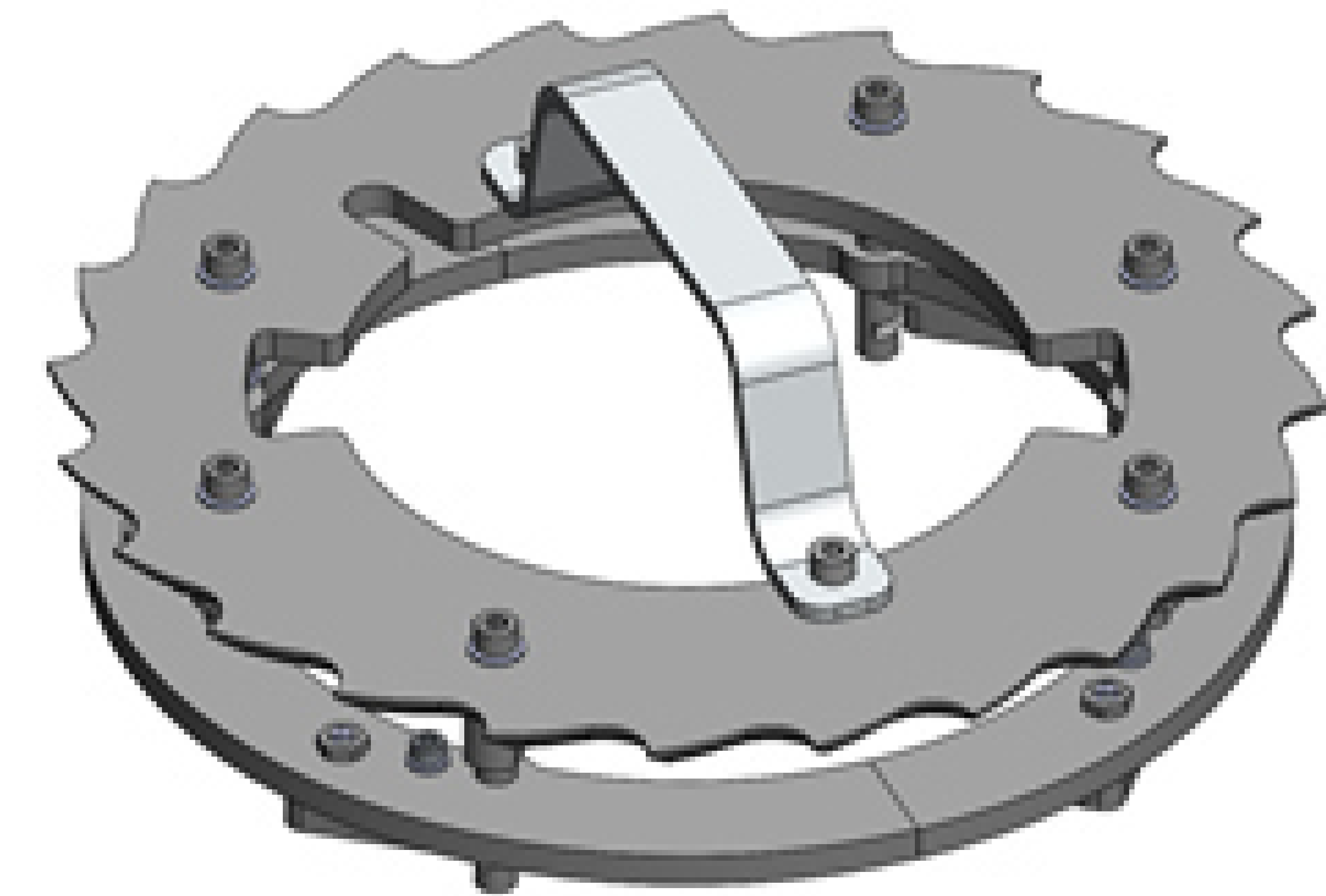
Entry wheel
