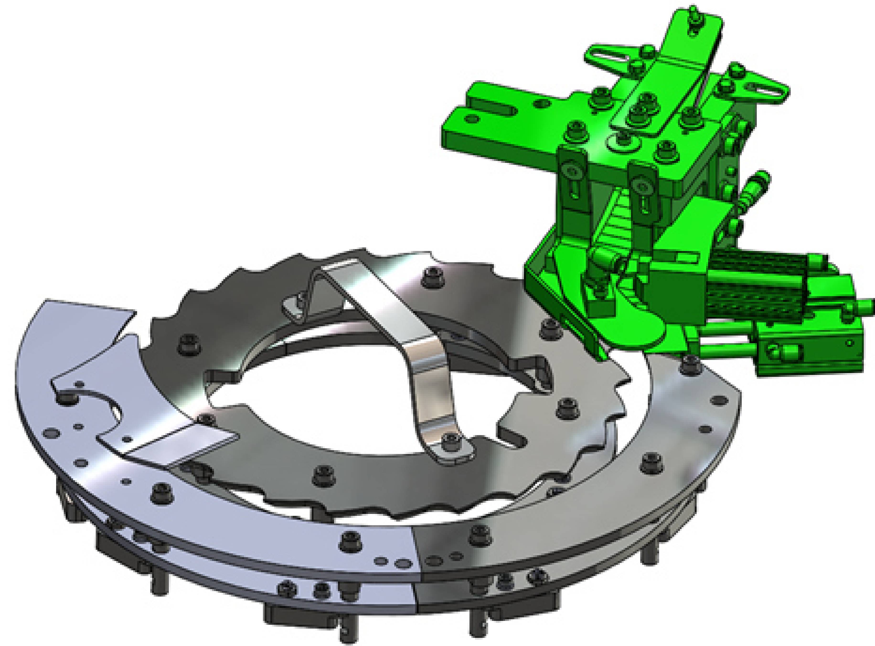
Entry guide
