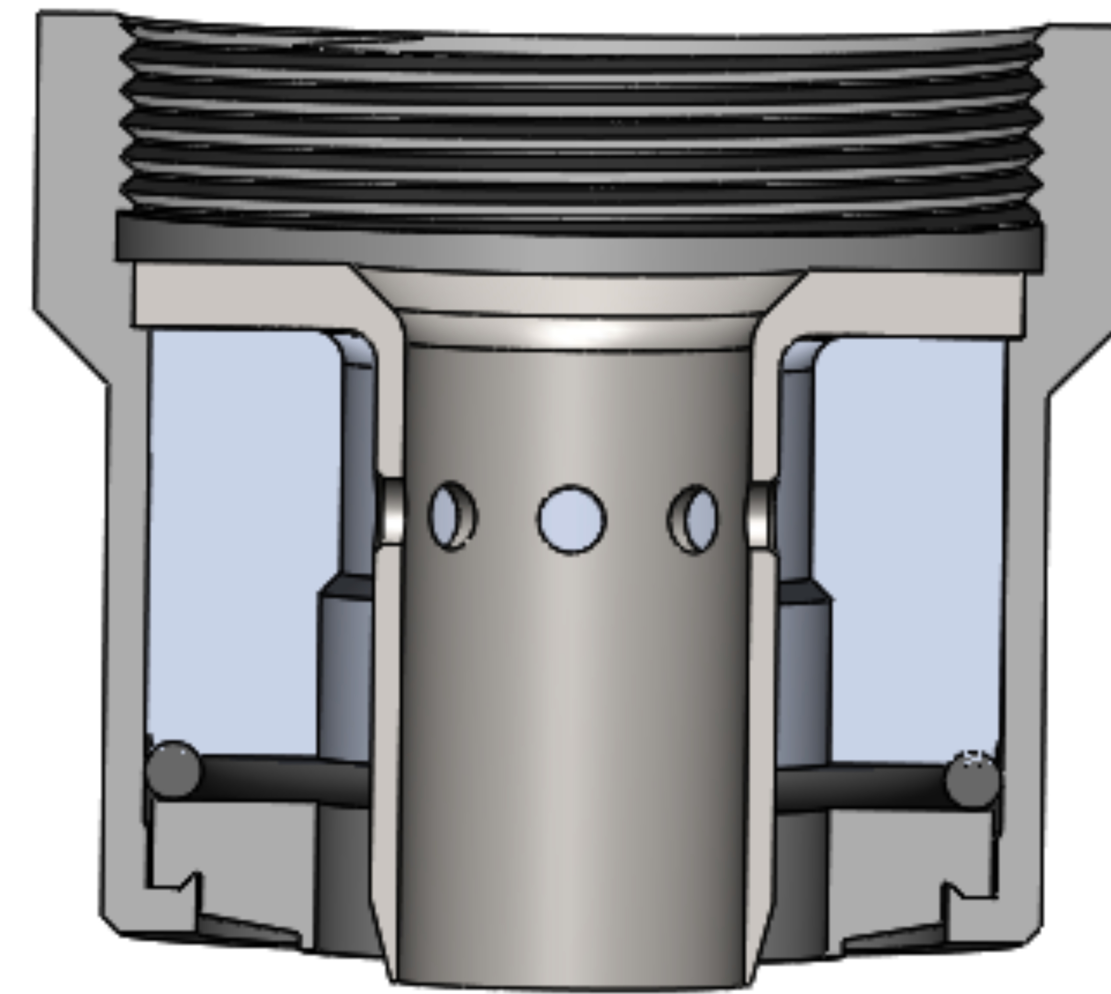
Blow nozzle bell
