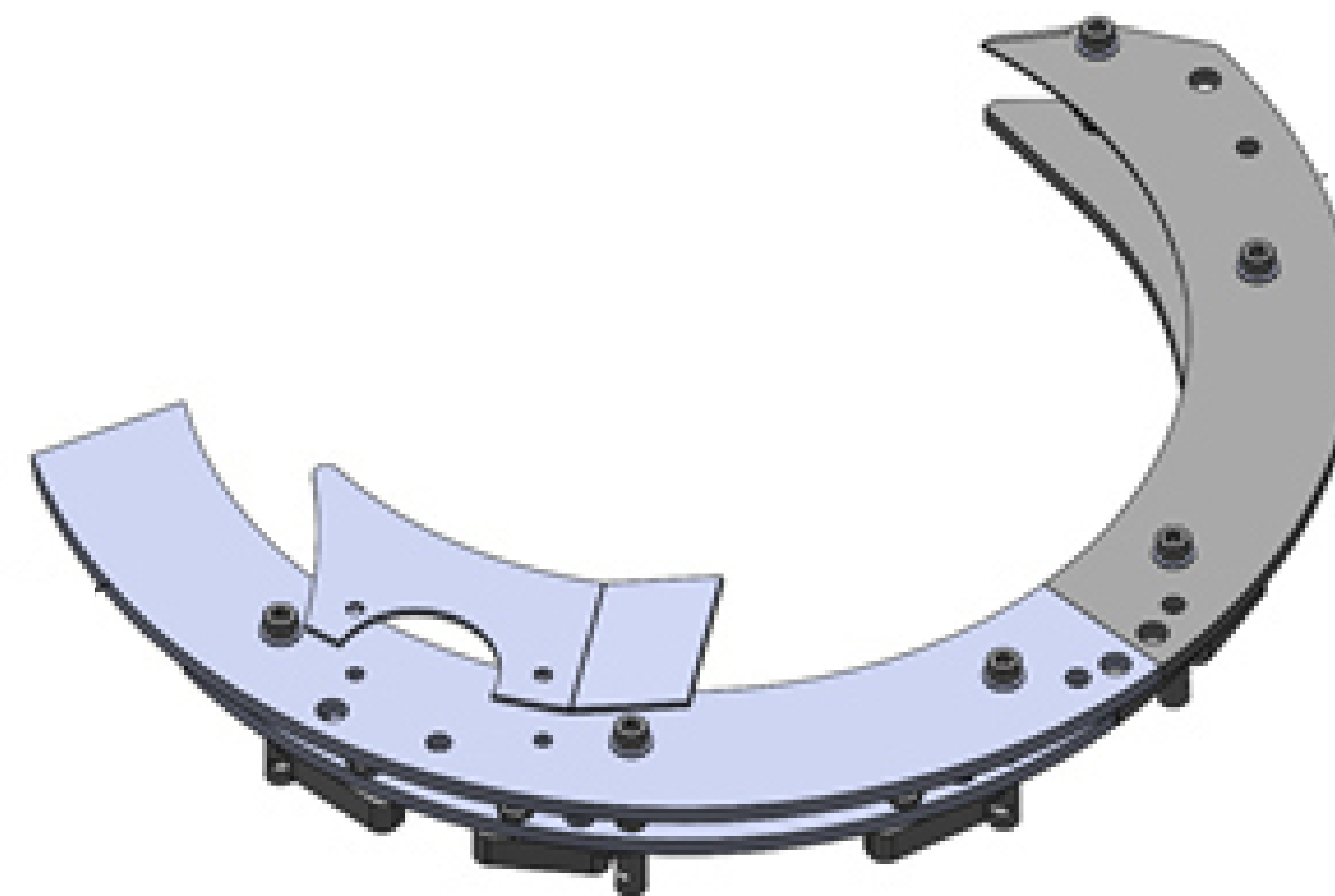
Entry guide
